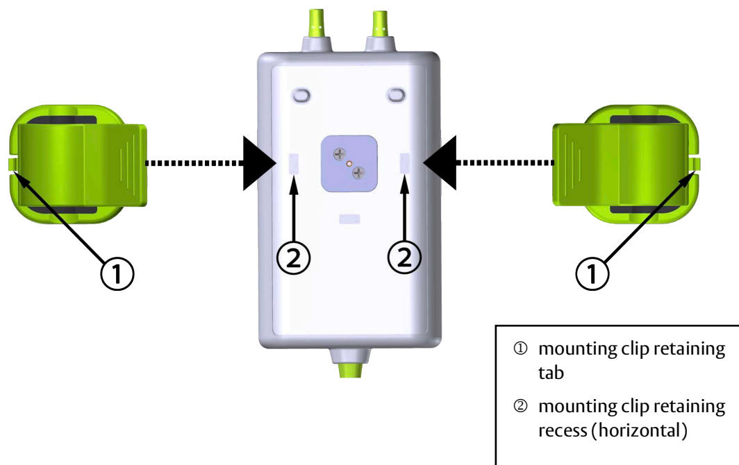
Figure 12-6 Attaching the mounting clip horizontally
