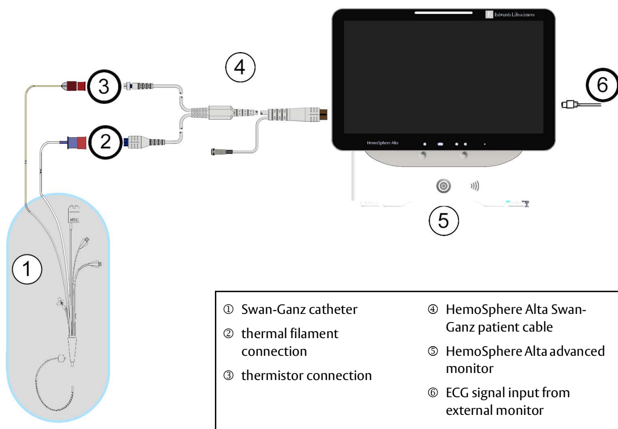
Figure 8-6 EDV/RVEF connection overview
