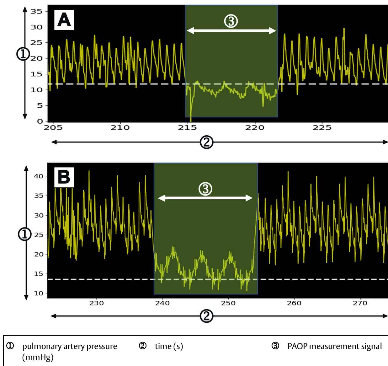
Figure 9-3 Example of Smart Wedge™ Algorithm PAOP measurement with spontaneous breathing (A) and mechanical ventilated (B) inputs
