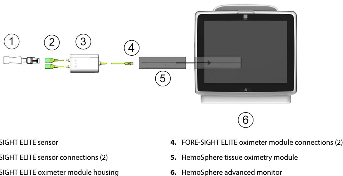
Figure 4-4: HemoSphere tissue oximetry module connection overview
