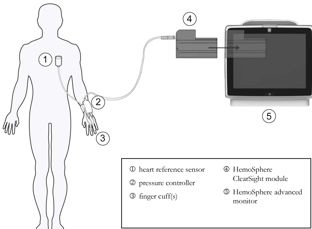
Figure 4-5 HemoSphere non-invasive system connection overview (wrist applied pressure controller)
