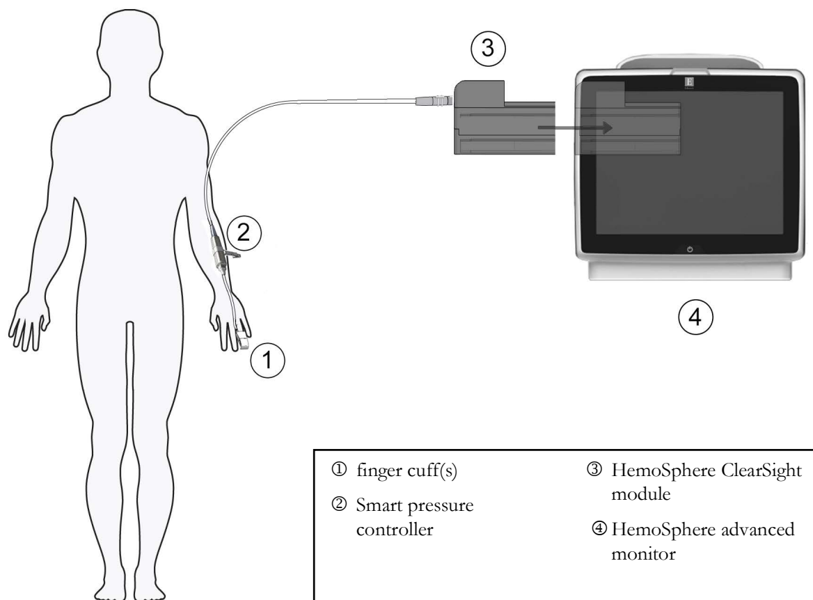
Figure 4-6 HemoSphere non-invasive system connection overview (Smart pressure controller)
