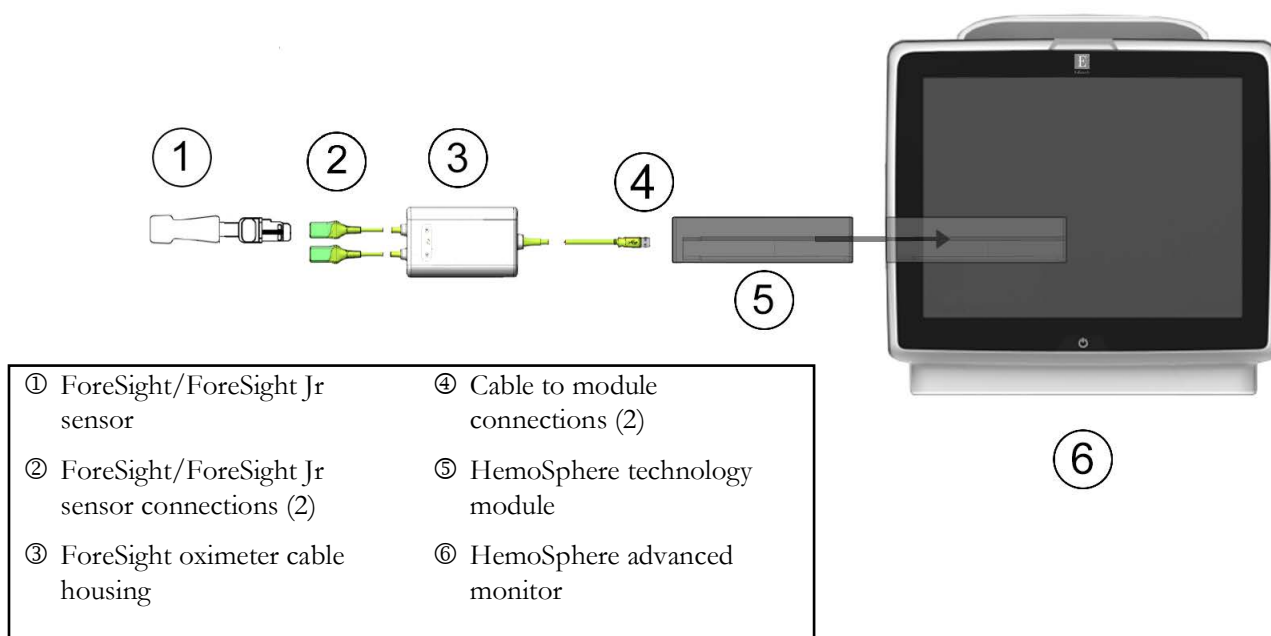
Figure 13-8 Tissue oximetry monitoring connection overview
