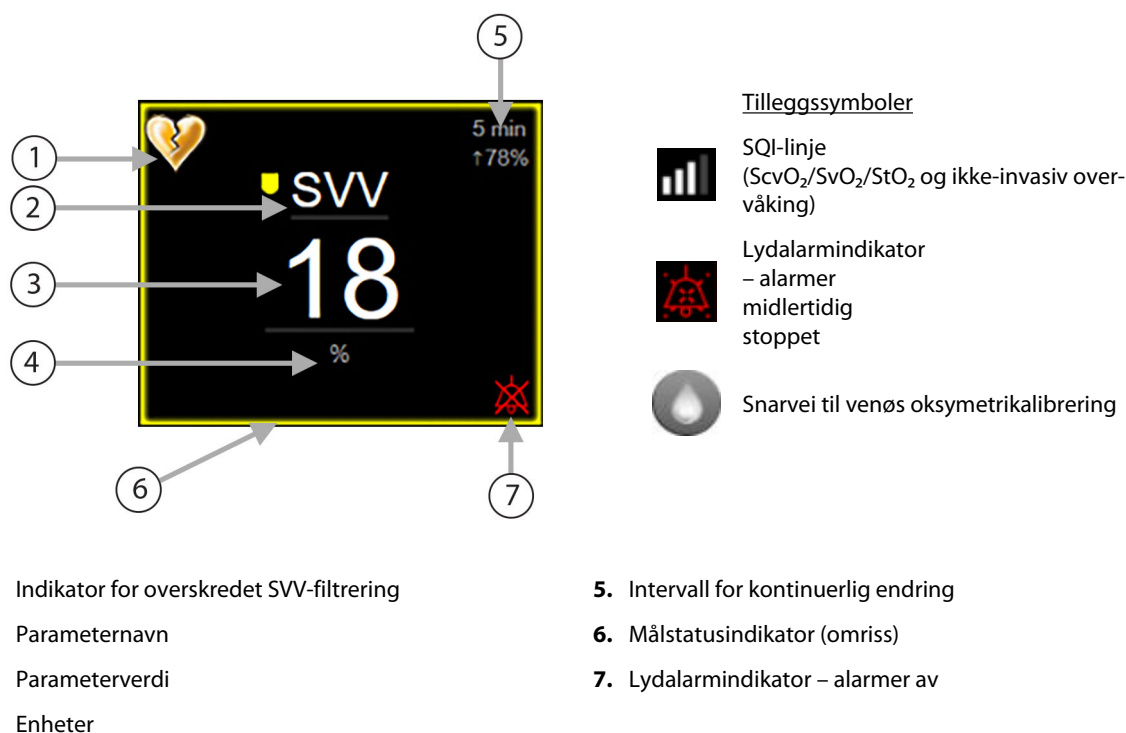
Figur 5-5: Parameterfelt
