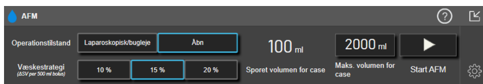
Figur 14-12: Dashboardet AFM
